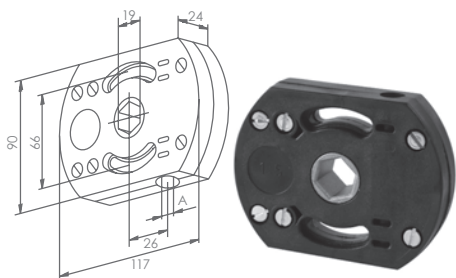
AT11002 Arganello "SYDNEY" 1:8 € 32,65
